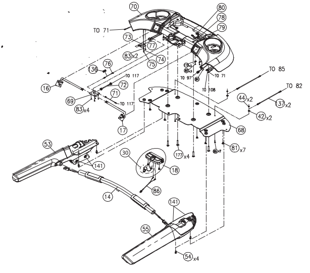
Detail view of Console Base
