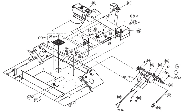
Detail View of Electrical Components
