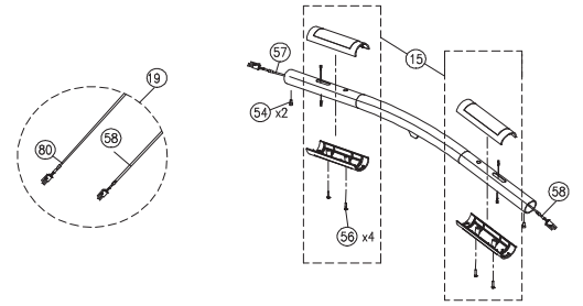
Detail view of Crossbar
